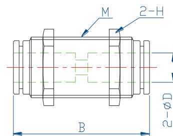
Bulkhead Union, BU
