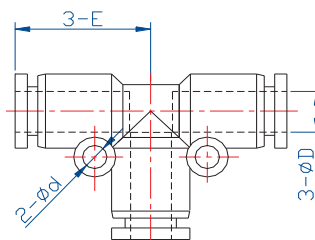
Tee Union, TU
