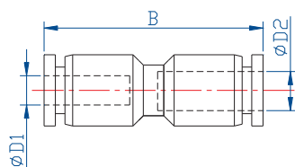
Reduced Union, RU
