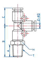
Run Tee, RT
