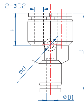
Reduced Branch, RB
