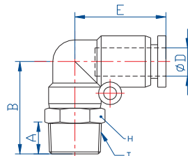
Male Elbow, ME
