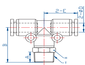
Branch Tee, BT
