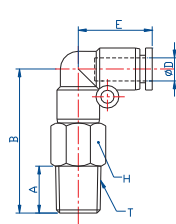
Extended Elbow, EE
